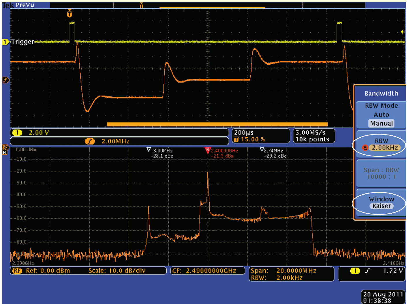
Figure A5. Kaiser Window in 2 kHz RBW.
