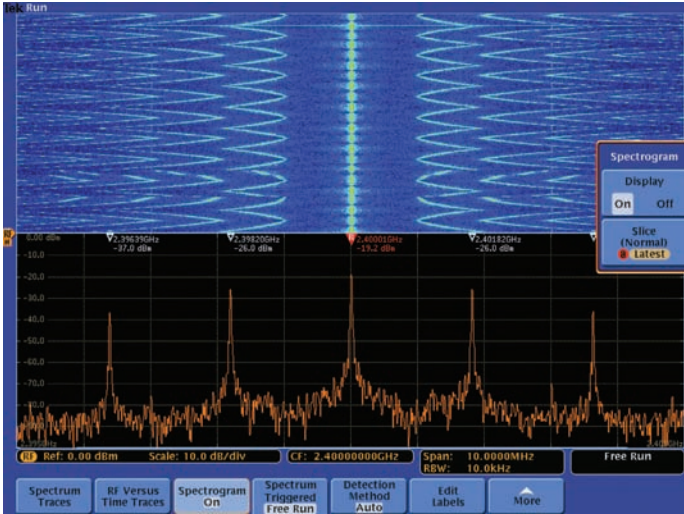
Figure 45. Spectrogram display shows the recorded spectrum history of a single.
