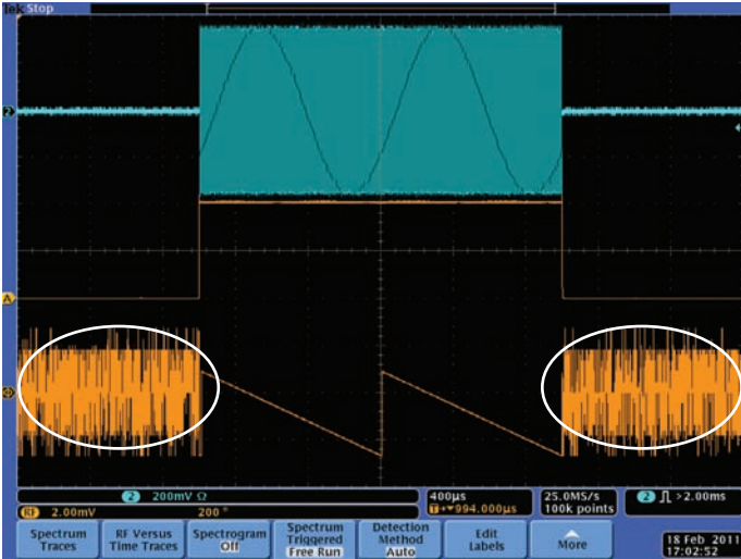
Figure 43. Phase vs. Time, Unblanked.
