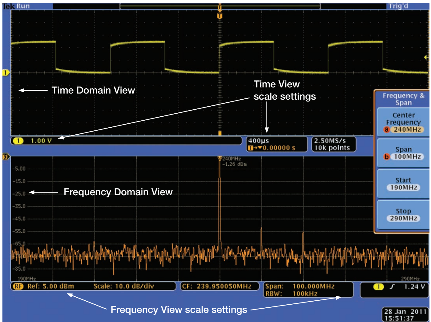
Figure 6. MDO4000 Display Overview for Time and Frequency Domain Views.
