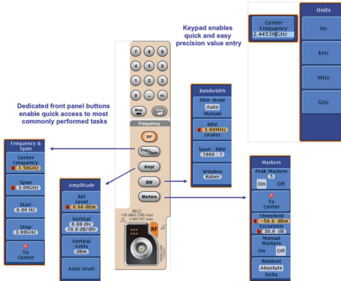
Figure 11. MDO4000 Front Panel.
