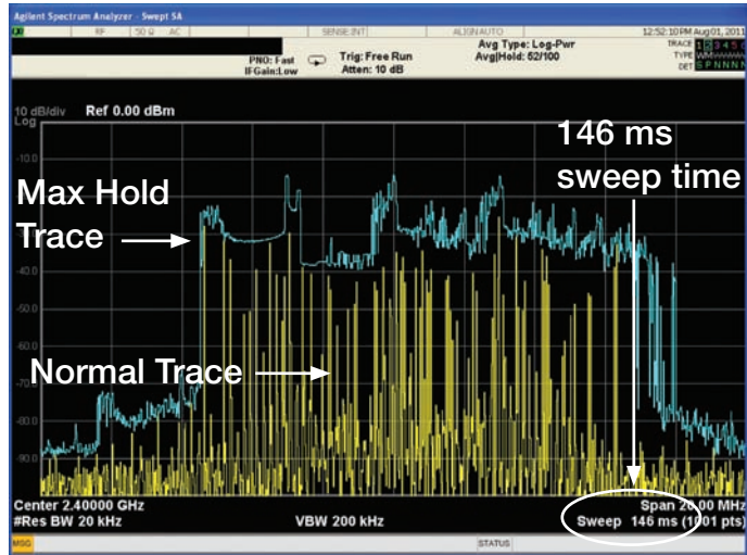
Figure 28. Spectrum analyzer measuring signal across 20 MHz of spectrum in 20 kHz RBW.
