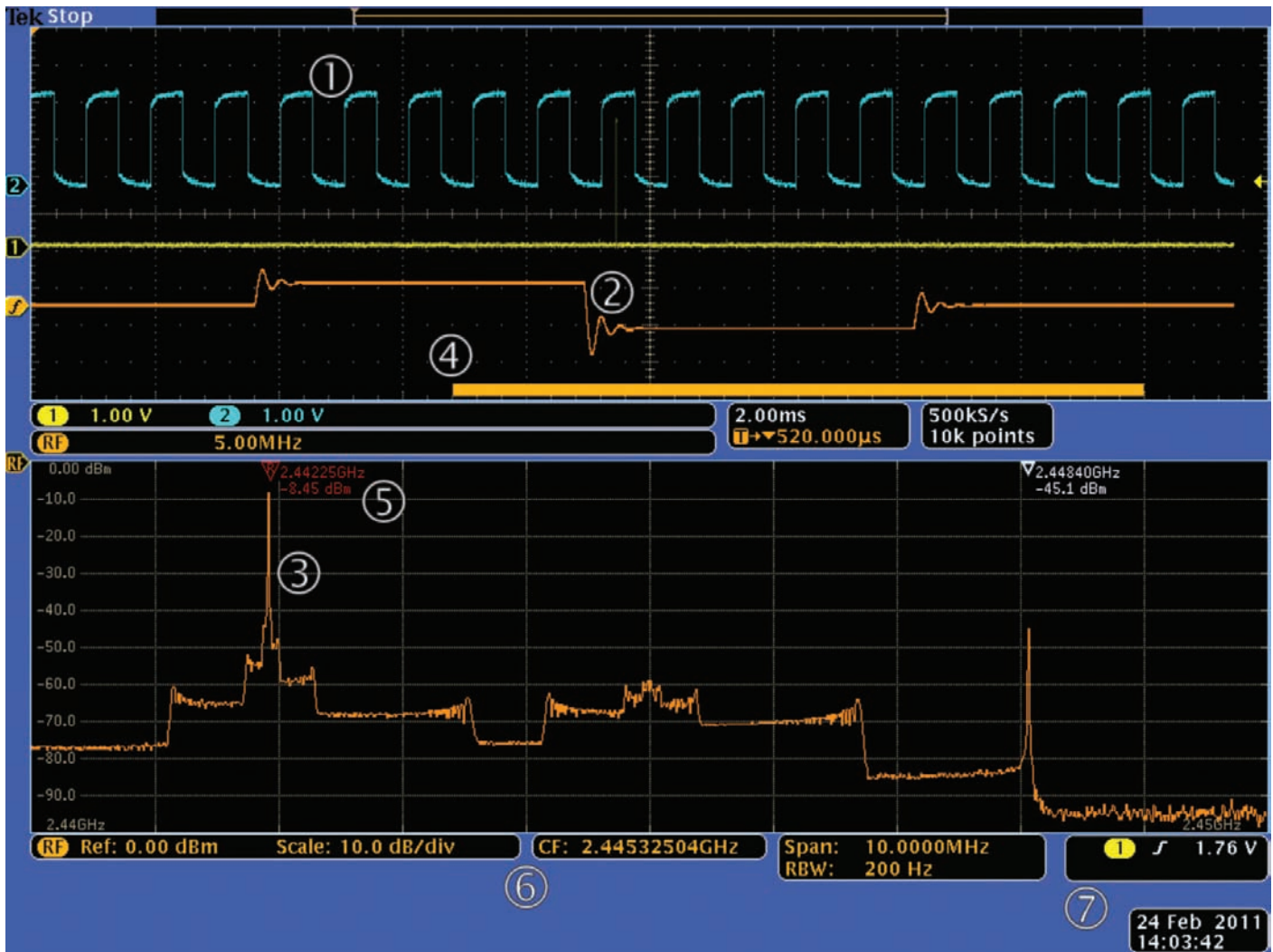
Figure 12. MDO4000 Display Elements.
