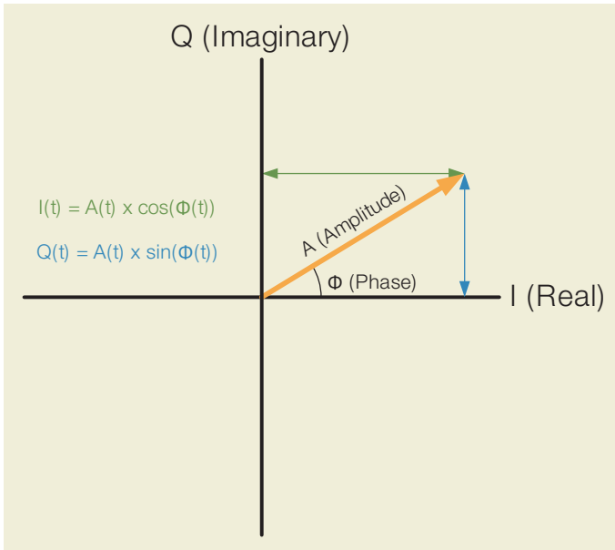
Figure 38. The IQ Data Plane.
