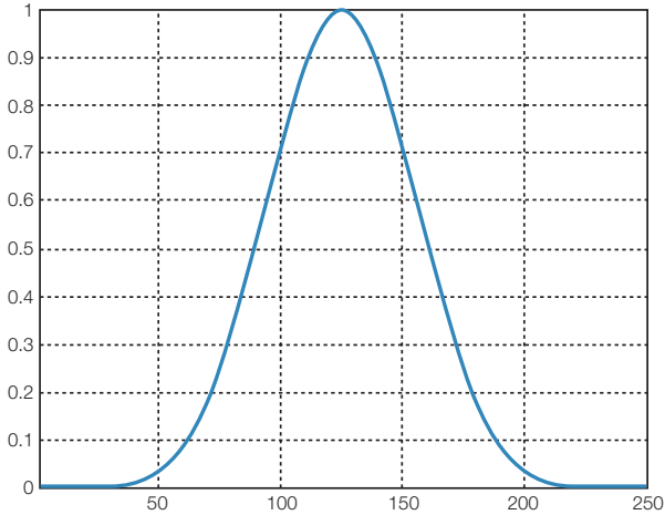
Figure A3. Kaiser Window in Time Domain - Horizontal is time samples, Vertical scale linear scale value.
