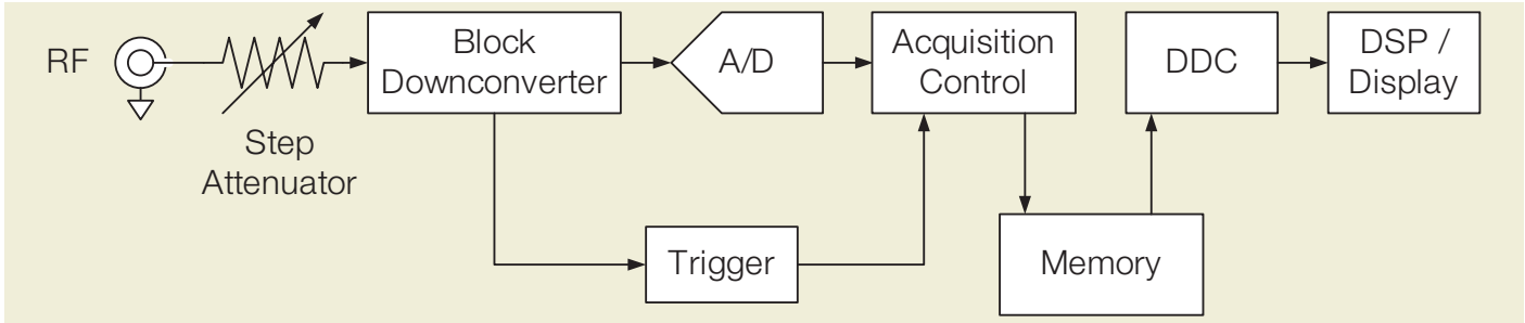
Figure 32. Simplified MDO4000 Block Diagram.
