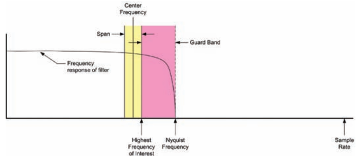
Figure 34. Low-Pass Filtering the Nyquist band.
