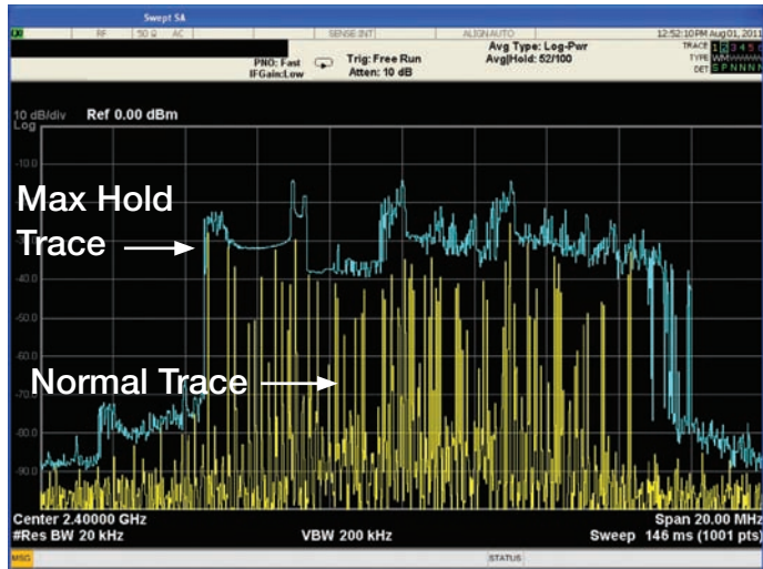
Figure 7. Spectrum analyzer measuring signal across 20 MHz of spectrum in 20 kHz RBW.
