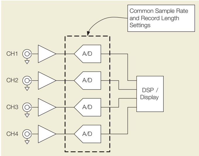
Figure 3. Typical Oscilloscope Architecture.
