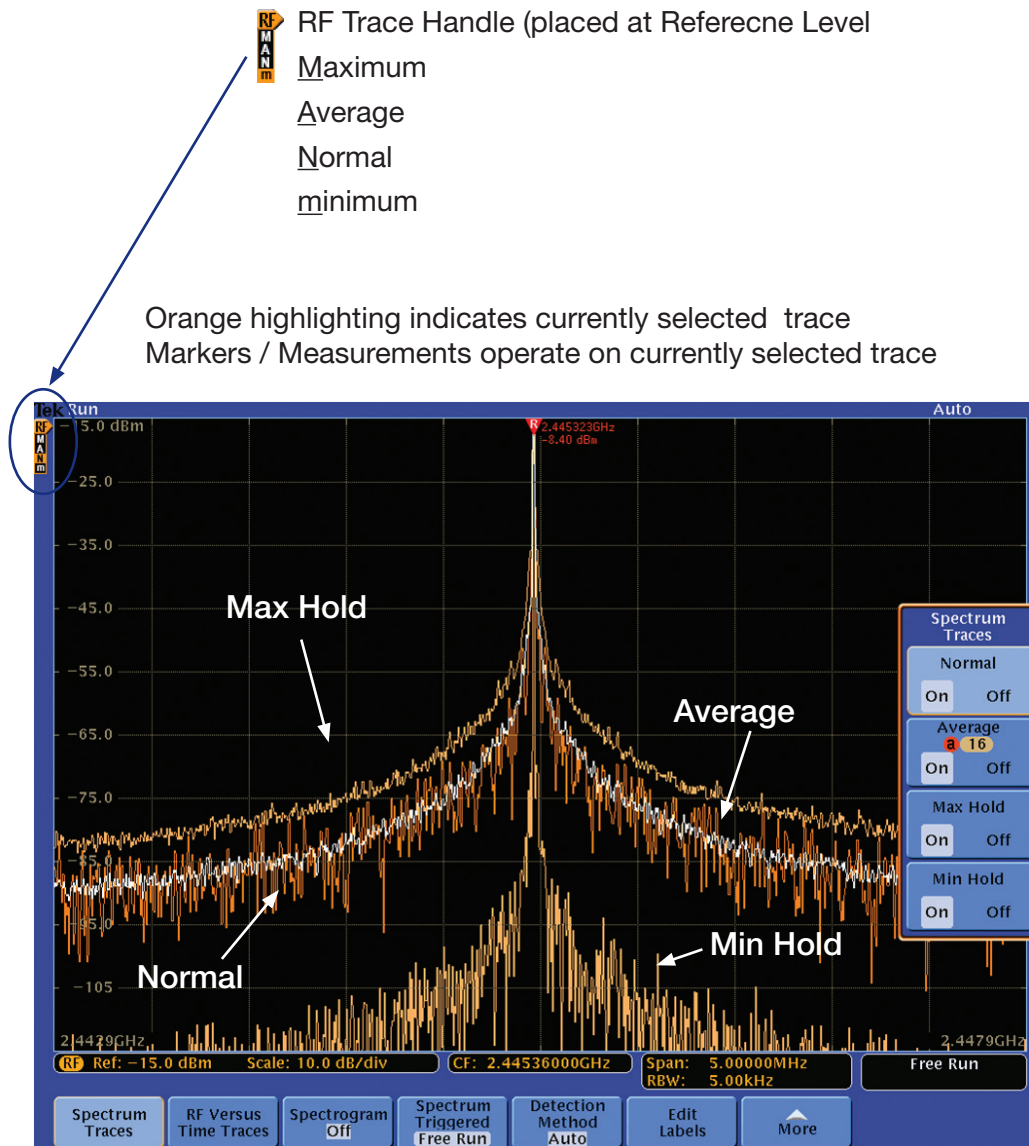
Figure 13. Spectrum Traces.
