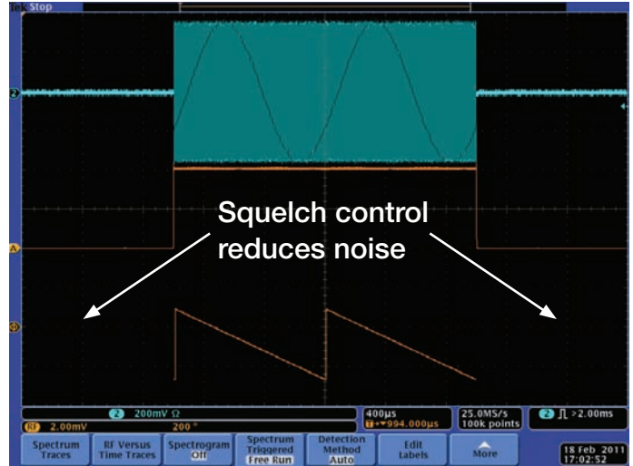
Figure 44. Phase vs. Time, Blanked.
