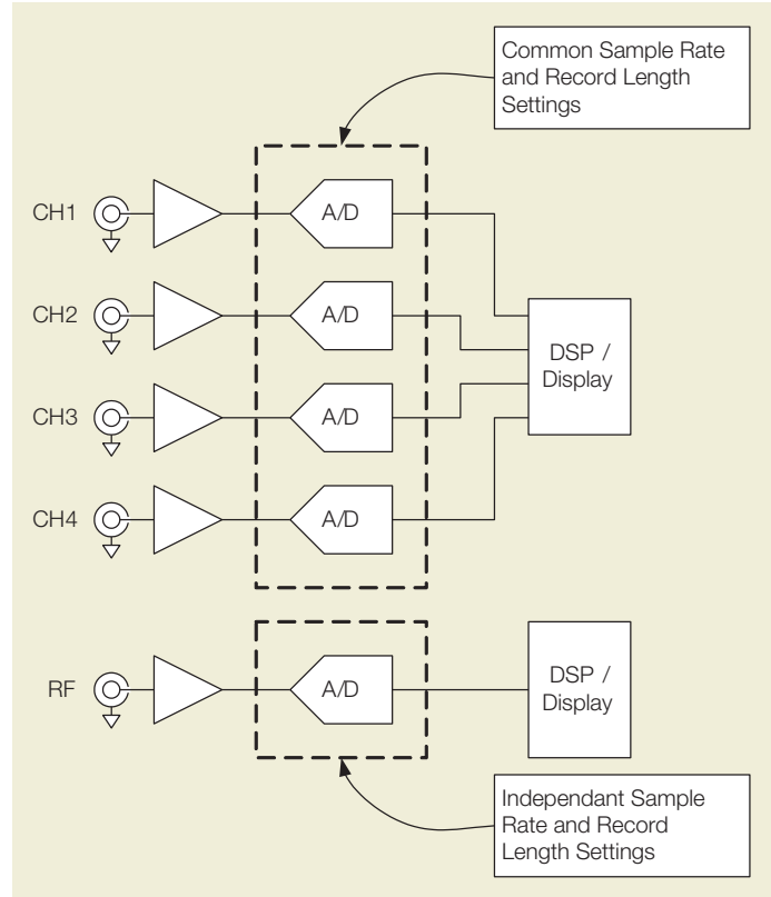
Figure 4. MDO4000 Simplified Acquisition system.
