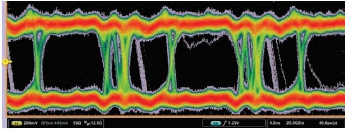
Figure 25. FastAcq visualization showing potential problems (in gray).
