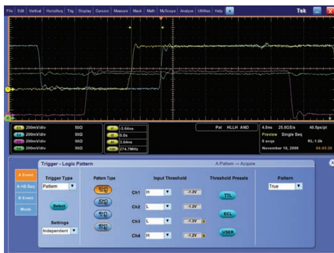
Figure 7a. Logic Pattern Triggering.
