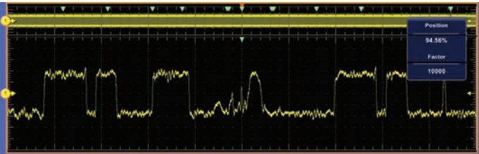
Figure 34. Results of Glitch and Window searches.
