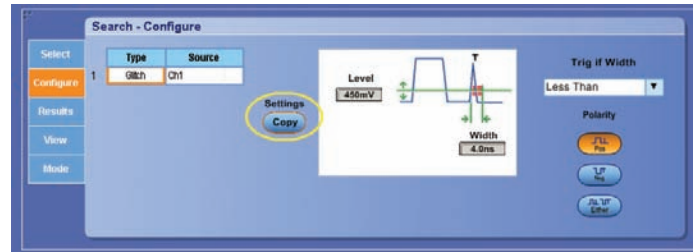
Figure 28. Glitch search method selected and copied to Advanced Search and Mark.
