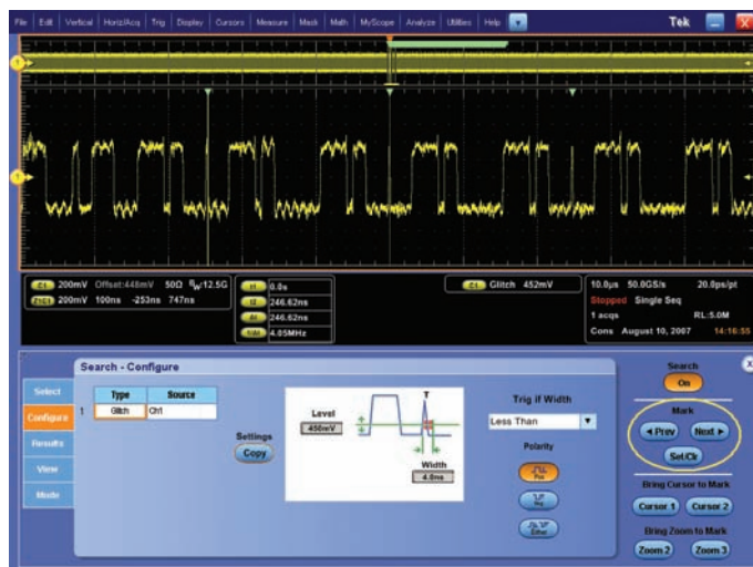
Figure 30. Display zoom.
