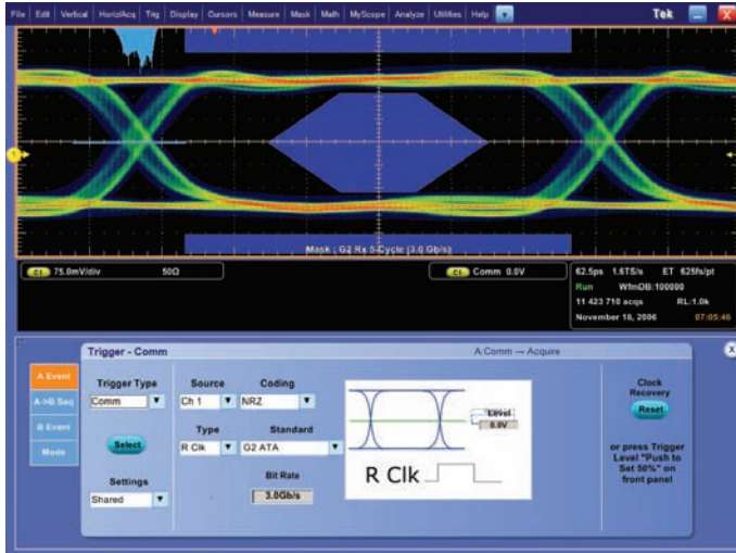
Figure 12. Communication Triggering.
