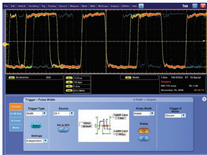
Figure 5b. Width Triggering.
