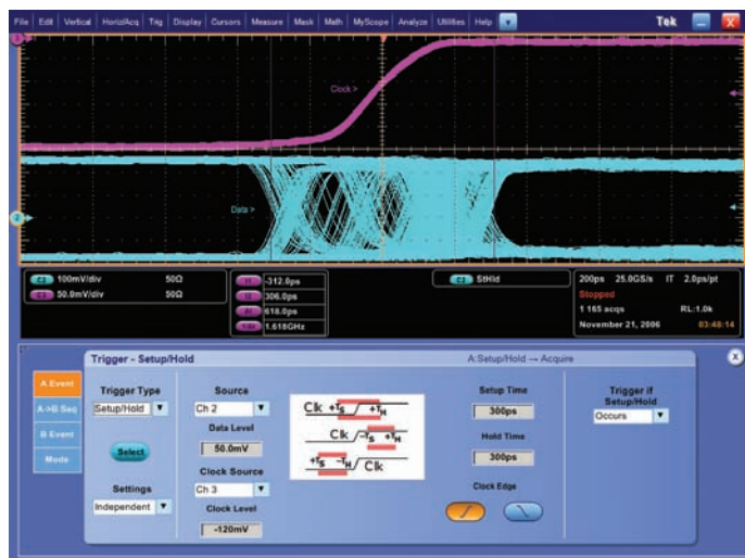
Figure 5f. Setup and Hold Triggering.
