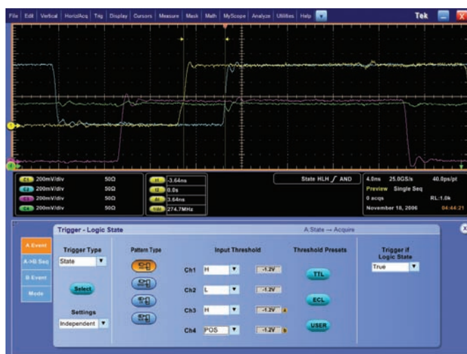
Figure 7b. Logic State Triggering.
