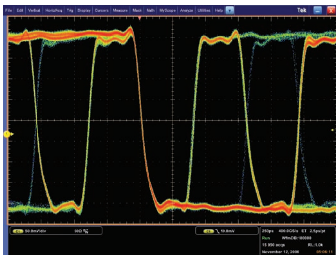
Figure 4b. Trigger Slope Negative.
