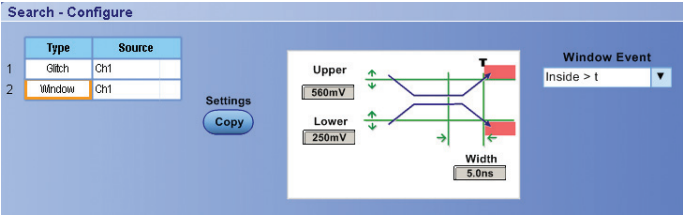
Figure 33. Window search.
