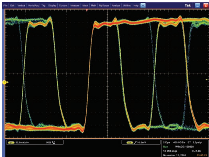
Figure 4a. Trigger Slope Positive.
