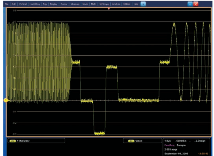
Figure 13. Video Triggering.
