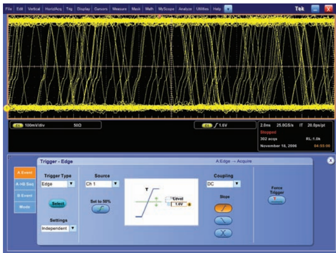
Figure 1. Untriggered Oscilloscope Display.
