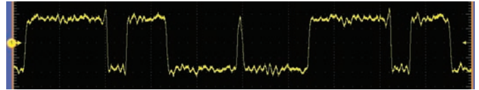
Figure 26. Glitch event detected using Pinpoint trigger type.
