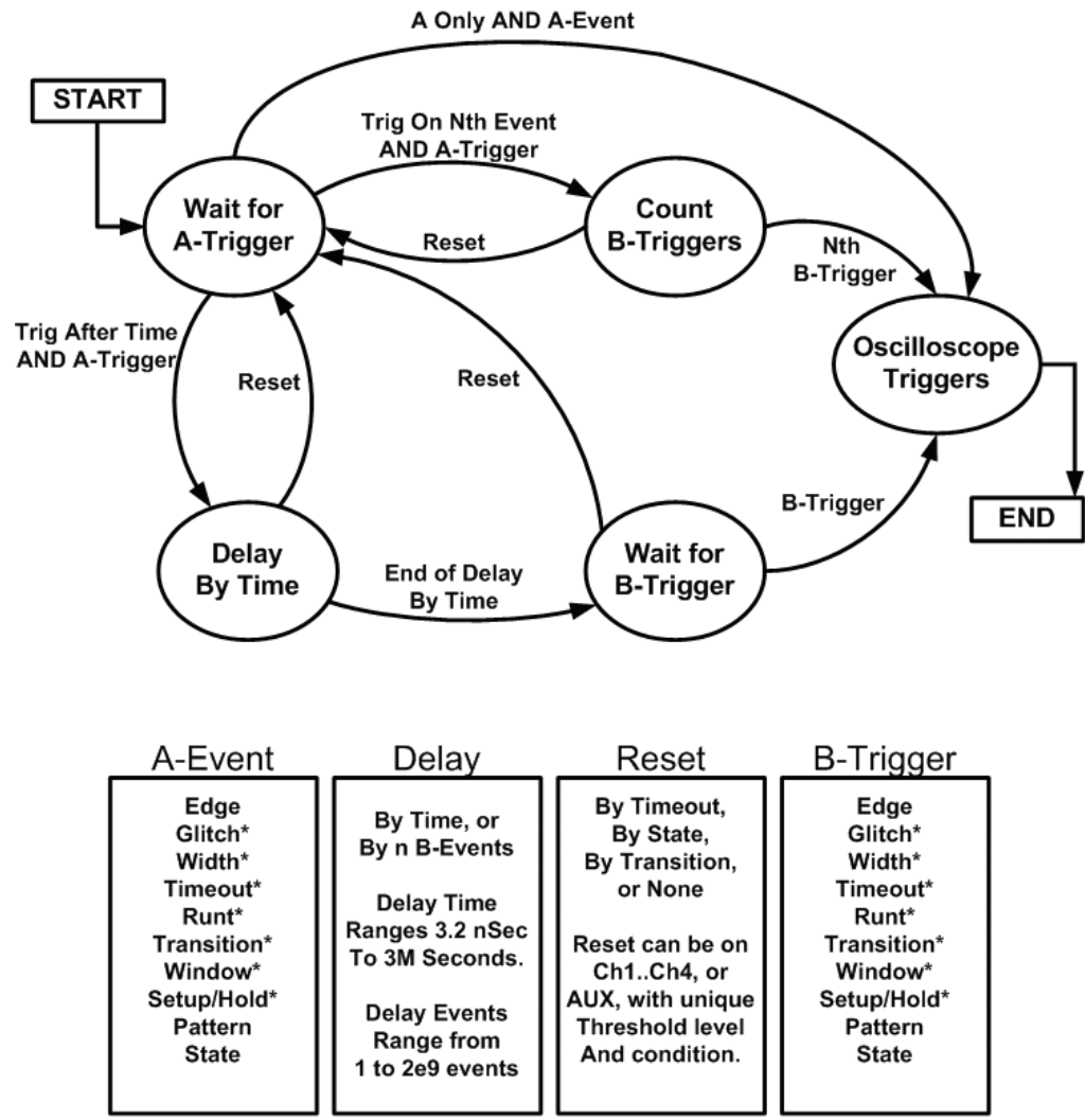
Figure 10. Pinpoint® Trigger State Machine.
