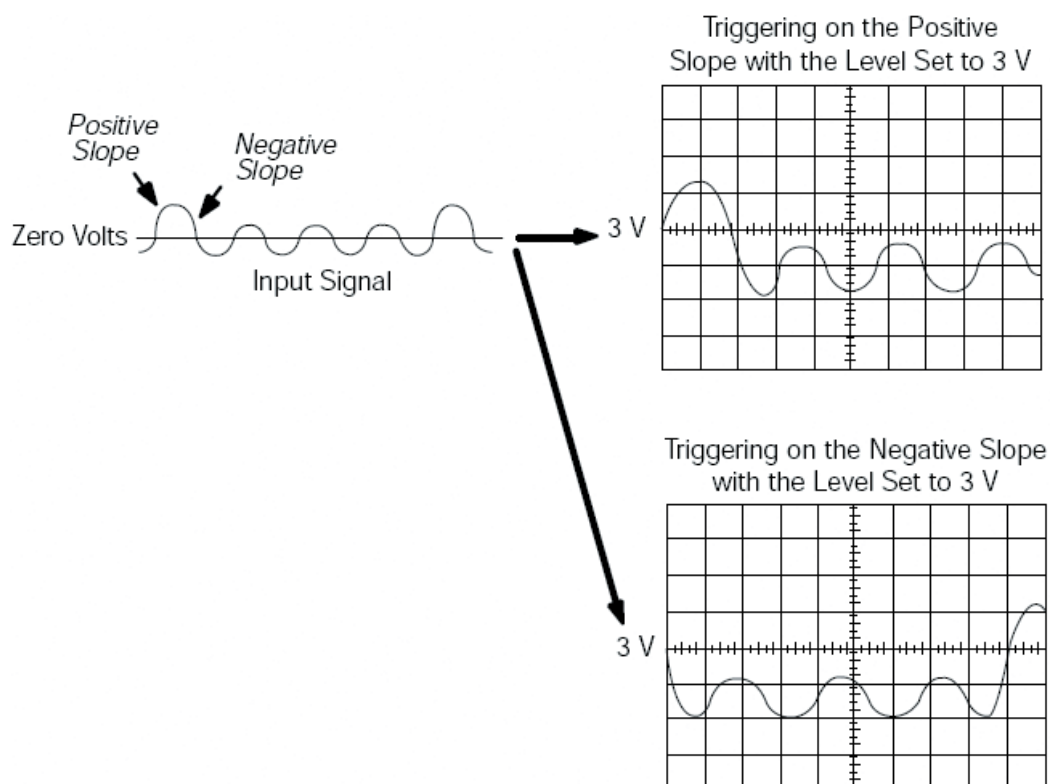
Figure 3. Trigger Level and Slope.
