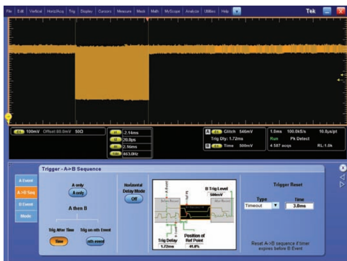
Figure 18. Beacon Width Violation Triggering.
