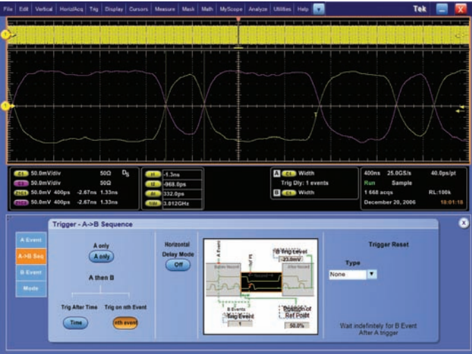
Figure 20. Lone Bit Pattern Trigger Setup.
