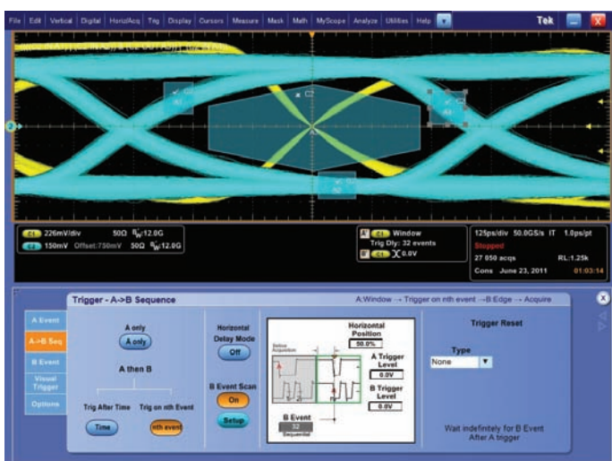
Figure 24. Visual Trigger on a Data Qualifier Eye for DDR3.
