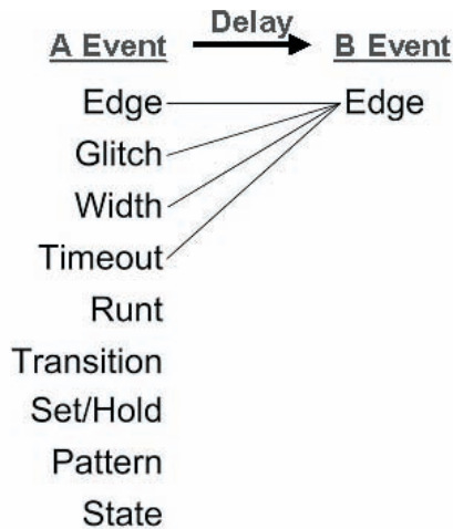
Figure 11a. Previous Generation Triggering - 17 trigger combinations.
