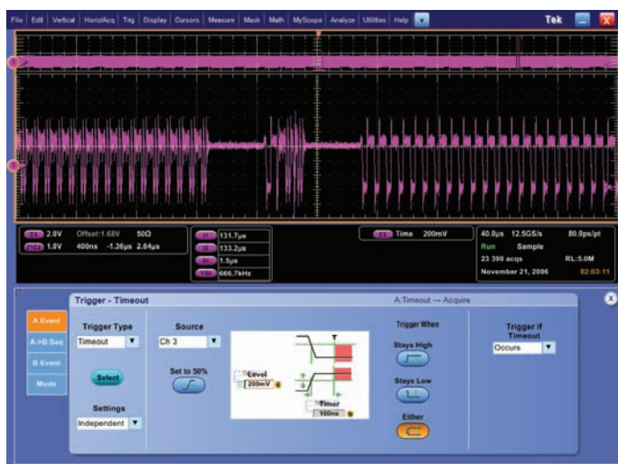
Figure 5d. Timeout Triggering.
