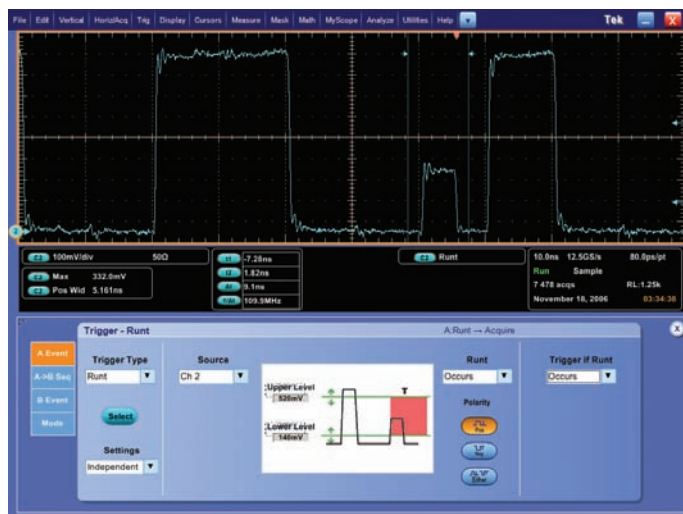
Figure 5c. Runt Triggering.
