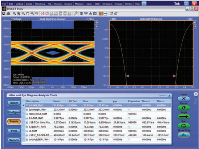
Figure 21. Lone Bit Pattern on DPOJET™.
